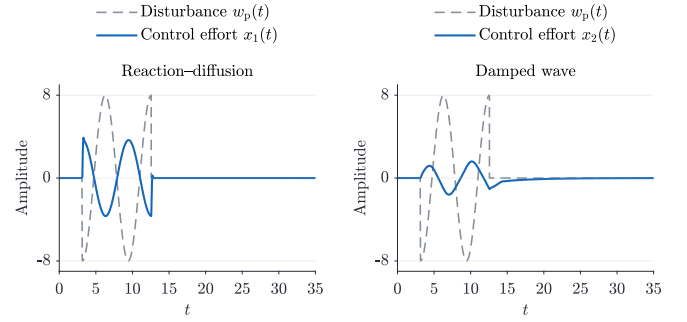
Figure 8: Disturbance and control effort for the reaction–diffusion equation (left) and damped wave equation (right). The dashed gray curve is w_p(t) .
