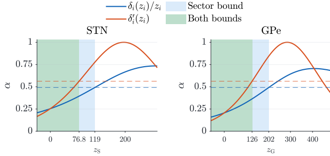
Figure 9: Sector quotients (blue) and differential slopes (orange) for the shifted STN and GPe nonlinearities. Dashed horizontal lines indicate \alpha_{\text{sec}}^* = 0.492 and \alpha_{\text{ZF}}^* = 0.562 . Blue shading denotes the sector-admissible interval; green shading denotes its intersection with the slope-admissible interval. Both intervals contain zero and extend to negative infinity. The additional x-axis ticks at the shaded boundaries mark the admissible upper limits.
